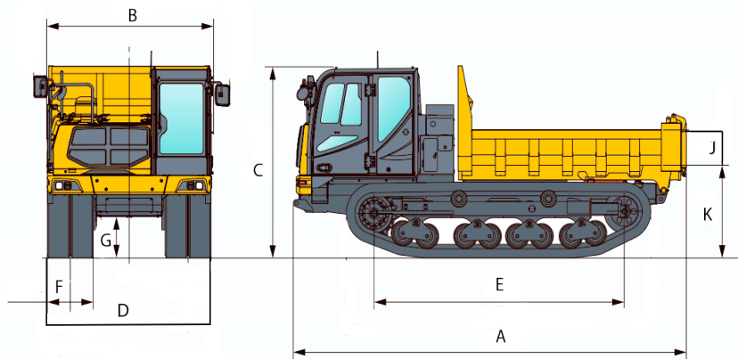
IC100-5 Crawler Carrier Working Ranges
